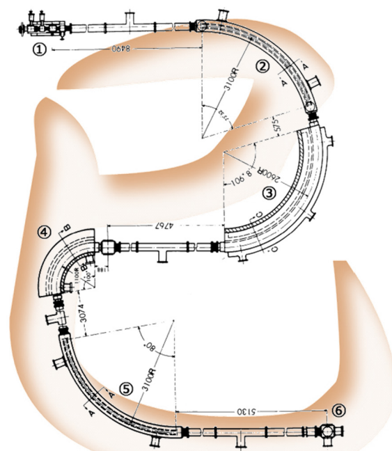
Schematic diagram of the "Orochi" mass spectrometer. 1: ion source, 2: first electric field, 3: first magnetic field, 4: second magnetic field, 5: second electric field, 6: final focus point. (after Katakuse et al., 1975, Mass Spectroscopy 23, 247-269)
